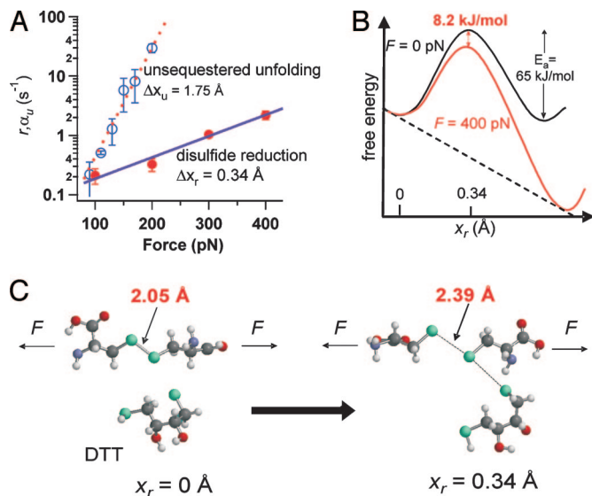
Fig. 5. Force sensitivity and bond lengthening in the thiol/disulfide exchange chemical reaction. (A) Semilogarithmic plot of the rate of thiol/disulfide exchange, r (filled circles) and of the unsequestered unfolding rate, r_u (open circles) as a function of the pulling force. The solid line is a fit of the equation r = A(\exp((F\Delta x_r - E_a)/k_B T))/[\text{DTT}] . The fit gave values of \Delta x_r = 0.34 Å and E_a = 65 kJ/mol (with A \approx 10^{12} \text{ s}^{-1} \text{ M}^{-1} ) for thiol/disulfide exchange. The dashed line fits the unsequestered unfolding rate with \alpha_u(F) = \alpha_u(0)\exp(F\Delta x_u/k_B T) obtaining \Delta x_u = 1.75 Å. (B) A simple illustration of the energy landscape of the thiol/disulfide exchange reaction under force. Our Bell-like model predicts that the transition state is located at 0.34 Å along the linear reaction coordinate, explaining the relative insensitivity of this reaction as compared with the unsequestered unfolding of the I27 protein. We calculate that applying 400 pN of force reduces the activation energy barrier for thiol/disulfide exchange by 8.2 kJ/mol. (C) Illustration of the thiol/disulfide exchange reaction between a DTT molecule and a disulfide bond under a stretching force. Only the two participating cysteine residues are shown for simplicity. The sulfur atoms are in green. The disulfide bond length increases from 2.05 Å initially (29) (Left) up to 2.39 Å at the transition state of an S_N2 reaction between the DTT molecule and the disulfide bond (Right).
