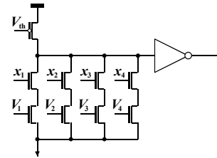
Figure 2. Implementation of the threshold function
